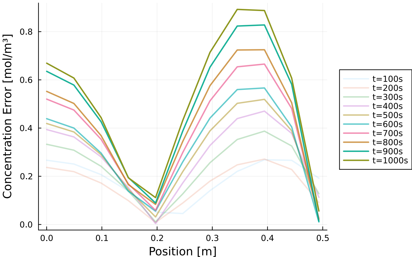
Concentration Error (sP2D vs P2D) - High Frequency Pulse
